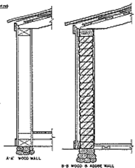
SECTIONS THRU EXTERIOR WALL SEE SHEET NO. 2 SCALE A
