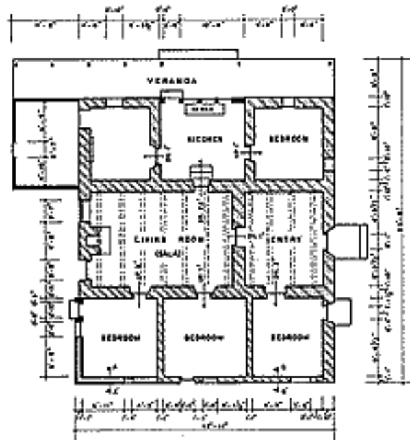
FLOOR PLAN SCALE D
